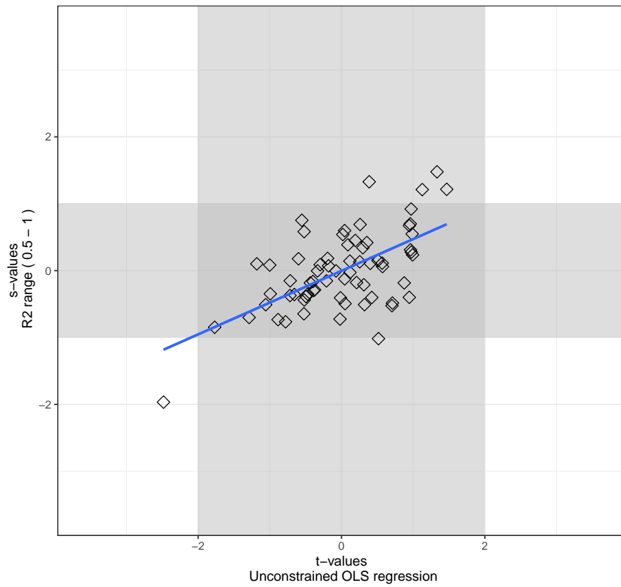
S-values x t-values Uncertain and Fragile Estimates Shaded
