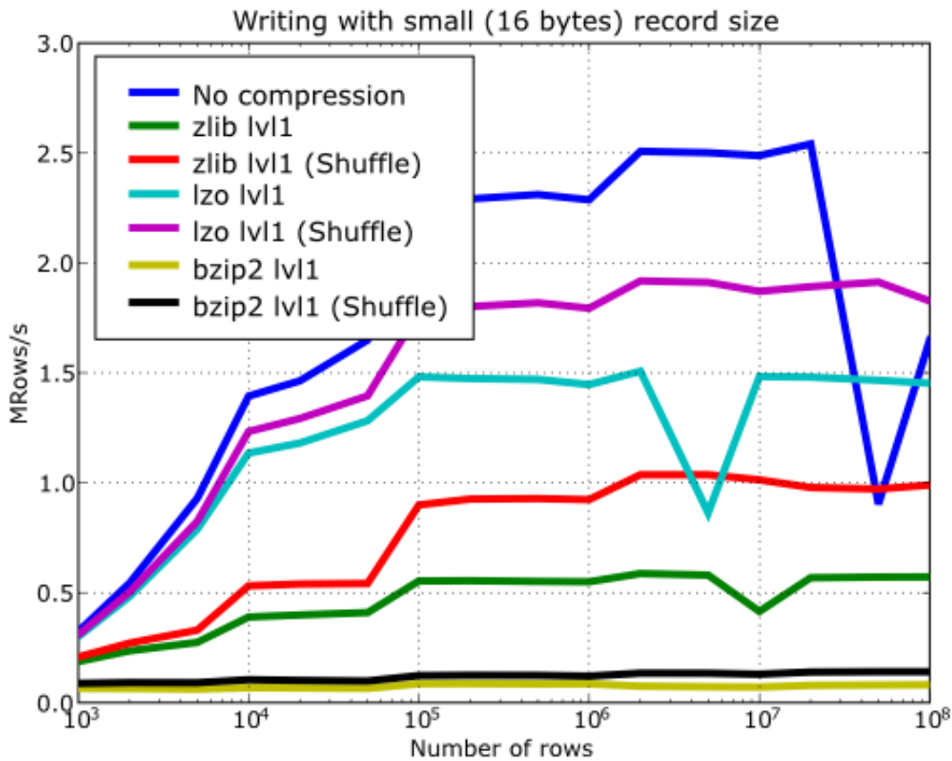
Figure 5.21: Figure 21. Writing with different compression libraries with and without the shuffle filter.
