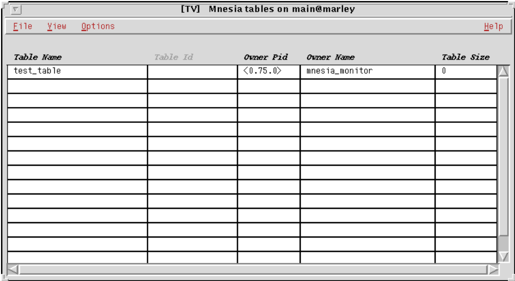
Figure 1.2: The TV Main Window, showing Mnesia tables.
