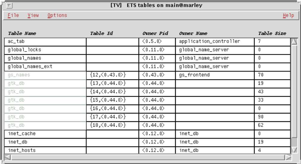
Figure 1.3: The TV Main Window, showing readable user and system tables.
