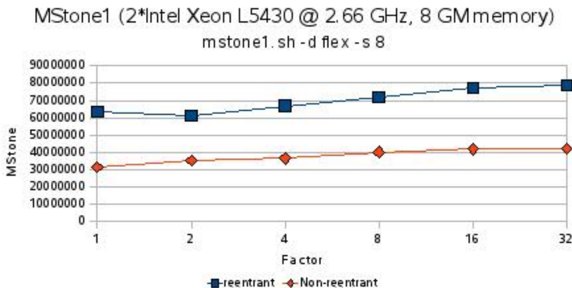
Figure 1.9: MStone1 with mstone1.sh -d flex -s 8
