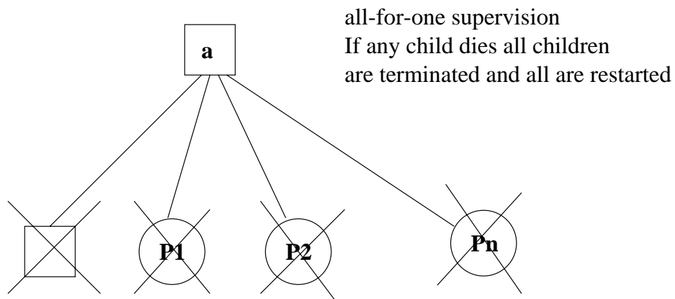
Figure 1.4: One_For_All Supervision
