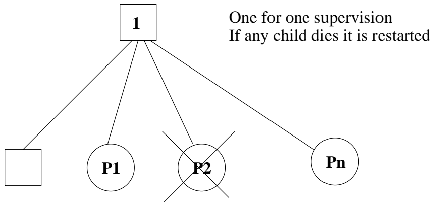
Figure 1.3: One_For_One Supervision
